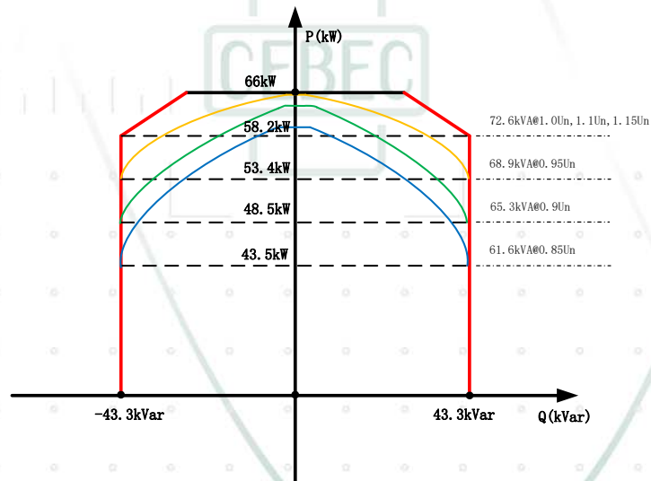
Figure 4. b. Voltage-dependent PQ diagram for MODEL iMars XG66KTR
