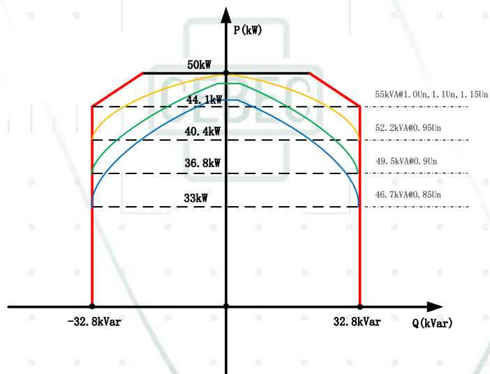
Figure 4.d Voltage-dependent PQ diagram for MODEL iMars XG50KTR
