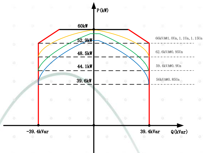
Figure 4.c Voltage-dependent PQ diagram for MODEL iMars XG60KTR
