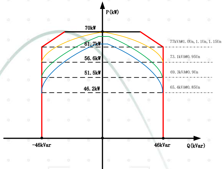
Figure 4 a. Voltage-dependent PQ diagram for MODEL iMars XG70KTRL
