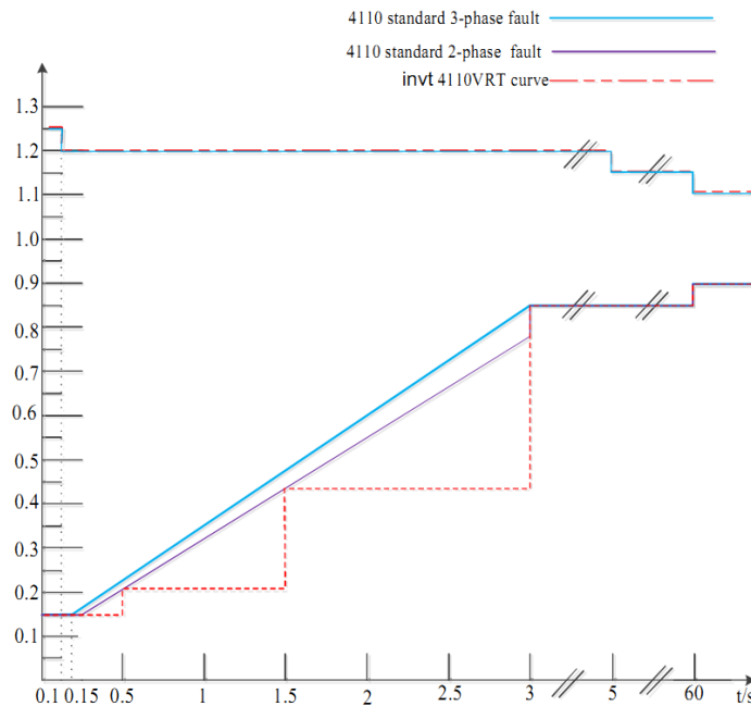
Figure 5 FRT limit curve for R Series PV
