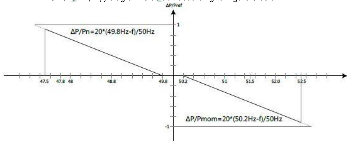
Figure 6 MODEL R Series PV P(f)-diagram
