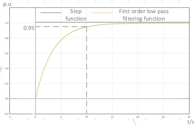
Figure 7 R SERIES reactive power control feature
