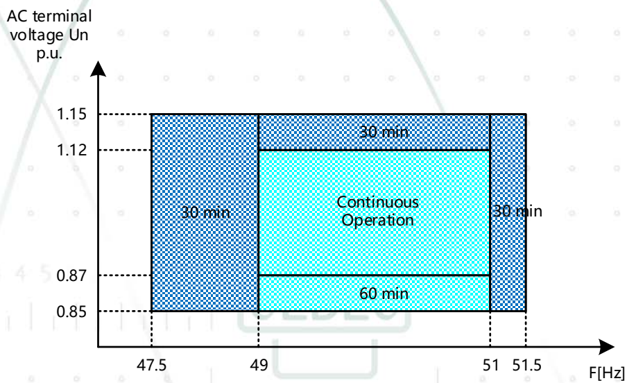
Figure 3 Quasi-stationary operation range for R SERIES PV inverter
